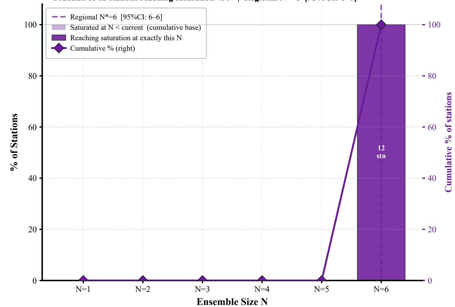
(d) r — Spatial Consensus Profile Fraction of 12 stations reaching saturation vs N | Regional N*=6 [95%CI: 6–6]
