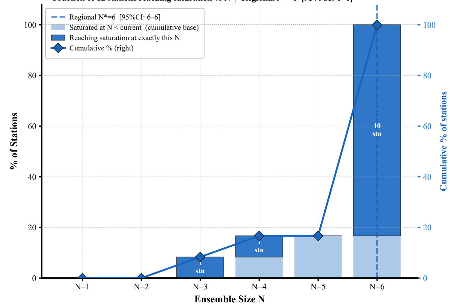
(b) KGE — Spatial Consensus Profile Fraction of 12 stations reaching saturation vs N | Regional N*=6 [95%CI: 6–6]
